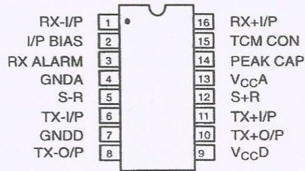
16 Lead PDIP (0.300 inch)
