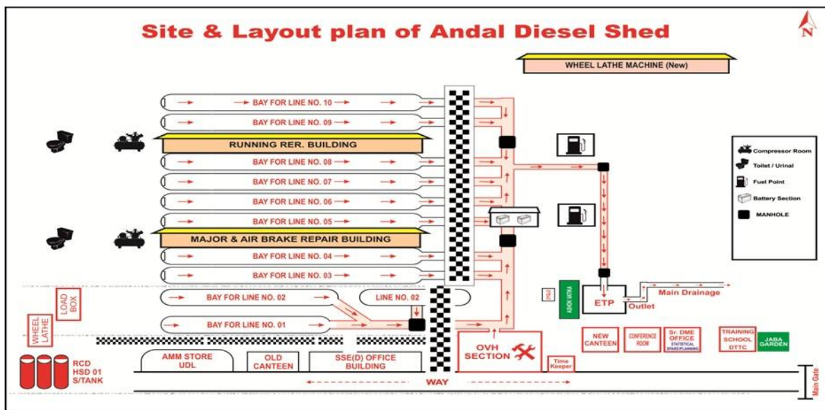
There are total 10 nos. of bay and length of each bay is approximately 190 ft.
